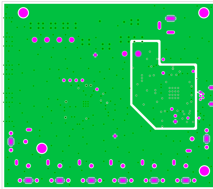
ADV7280AMEBZ Eval Board Rev. A (Primary Side View) Power Plane – Layer 3
