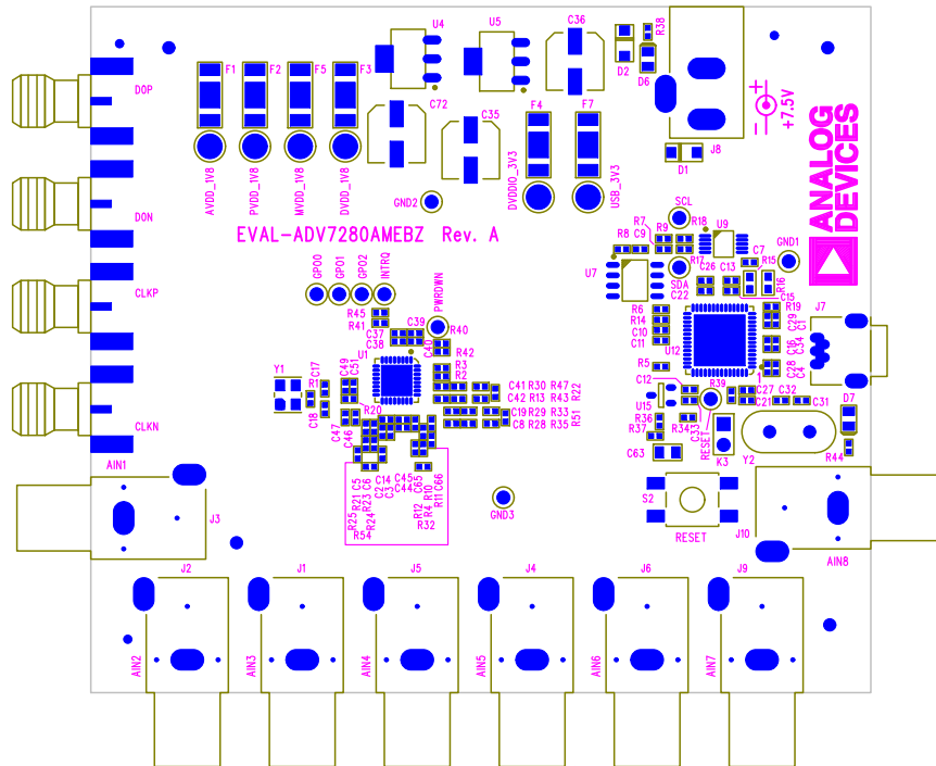
ADV7280AMEBZ Eval Board Rev. A (Primary Side View)
