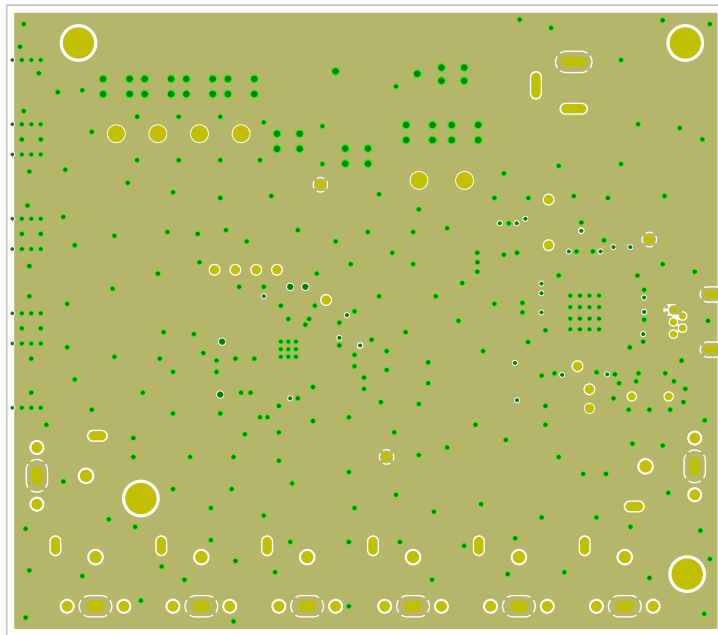
ADV7280AMEBZ Eval Board Rev. A (Primary Side View) Ground Plane - Layer 2
