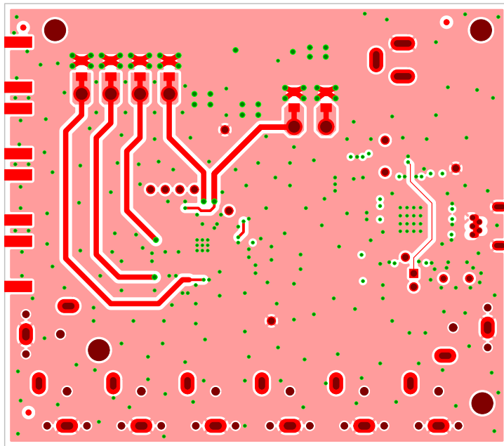
ADV7280AMEBZ Eval Board Rev. A (Primary Side View) Secondary Side - Layer 4
