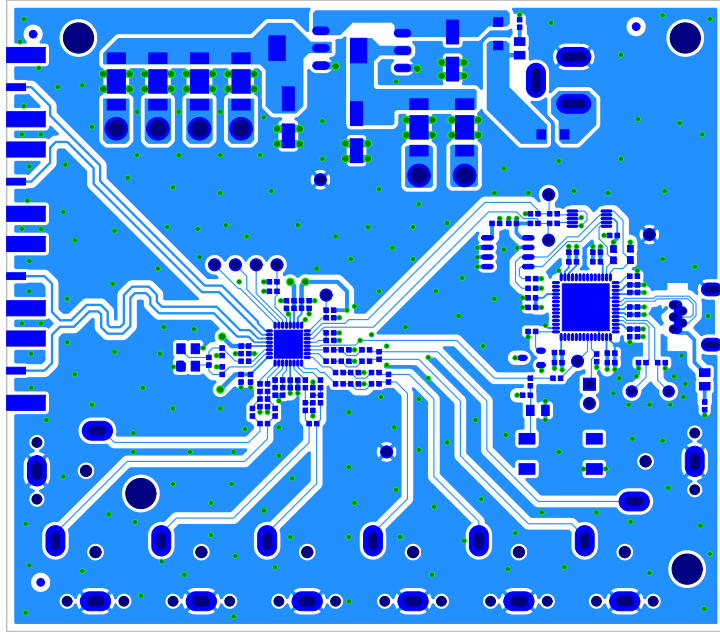
ADV7280AMEBZ Eval Board Rev. A (Primary Side View) Primary Side - Layer 1
