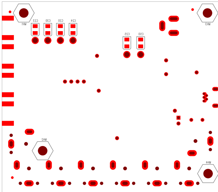
ADV7280AMEBZ Eval Board Rev. A (Primary Side View)
