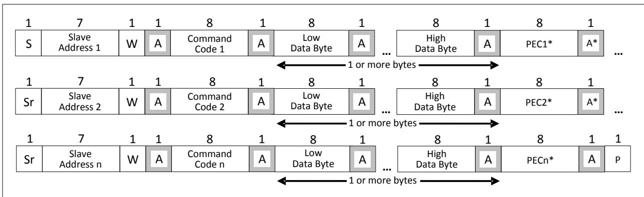
Figure 31: Group Command
