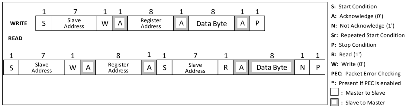
Figure 24: I2C Format
