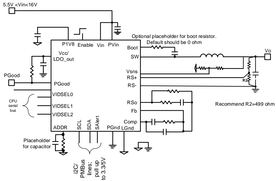
Figure 5: Using the internal LDO, V_o > 2.555V
