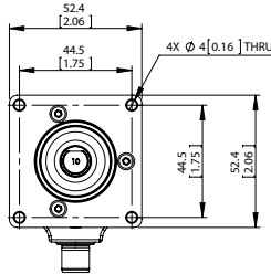
SQUARE FLANGE
